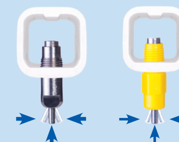
LUBING TOP-Nipple Art. 4022 (left) and the TOP-Combinipple Art. 4024-00 (right) with sideways action for rearing.
